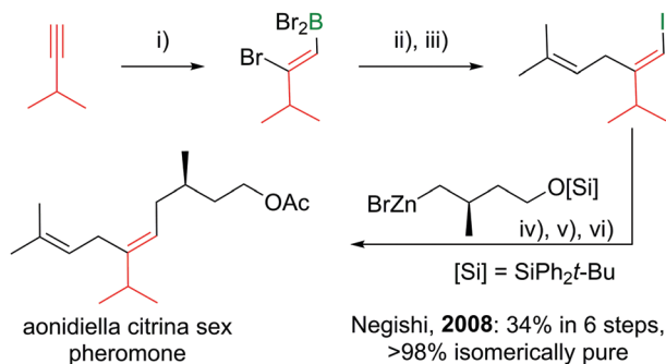
Scheme 25 Example of a natural product synthesis sequence based on haloboration. Reagents and conditions: (i) \text{BBr}_3 , DCM, -78\text{ }^\circ\text{C} to 23\text{ }^\circ\text{C} , 1 h; (ii) \text{Me}_2\text{C}=\text{CH}-\text{CH}_2\text{ZnBr} , \text{Pd}(\text{PPh}_3)_2\text{Cl}_2 (1 mol%), THF, 23\text{ }^\circ\text{C} , 2 h; (iii) \text{I}_2 , NaOAc, THF/ \text{H}_2\text{O} , 23\text{ }^\circ\text{C} , 1 h; (iv) zinc organyl, \text{Pd}(\text{PPh}_3)_4 (1 mol%), THF, 23\text{ }^\circ\text{C} , 5 h; (v) [\text{n-Bu}_4\text{N}]\text{F} , THF, 23\text{ }^\circ\text{C} , 1 h; (vi) \text{Ac}_2\text{O} , pyridine, DCM, 23\text{ }^\circ\text{C} , 12 h.
