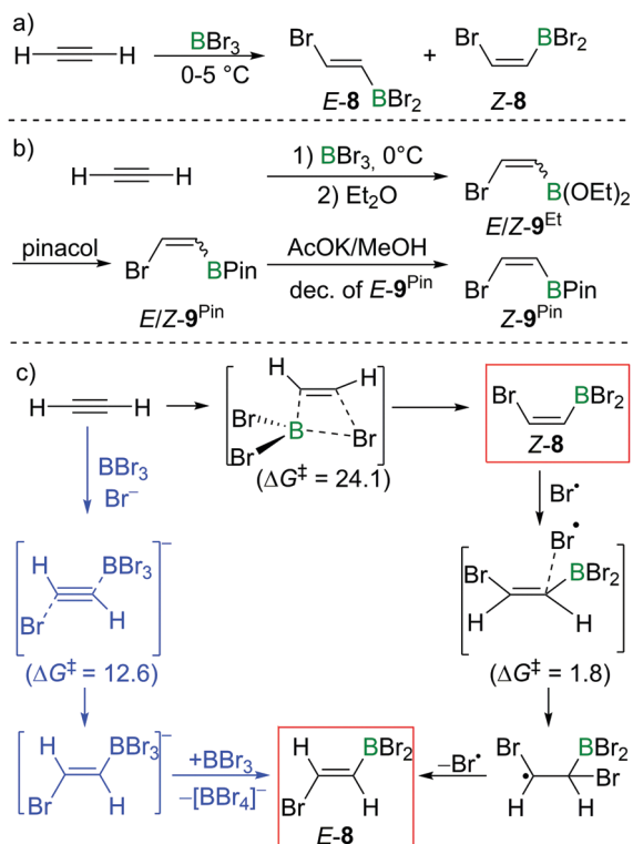
Scheme 8 (a) Reaction of acetylene with \text{BBr}_3 . (b) Brønsted-acid-free workup conditions allow for the selective isolation of Z -9 Pin . (c) Possible reaction pathways and energies ( \text{kcal mol}^{-1} ) of acetylene bromoboration.
