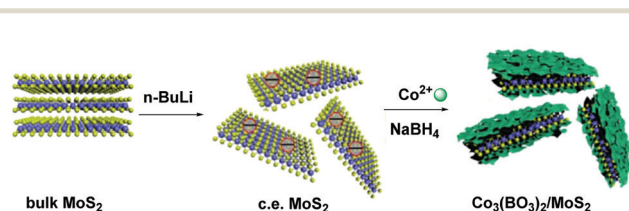
Fig. 12 Preparation of Co_3(BO_3)_2/MoS_2 hybrids. Reproduced in part with permission from ref. 29. Copyright © 2020 Elsevier Ltd.
