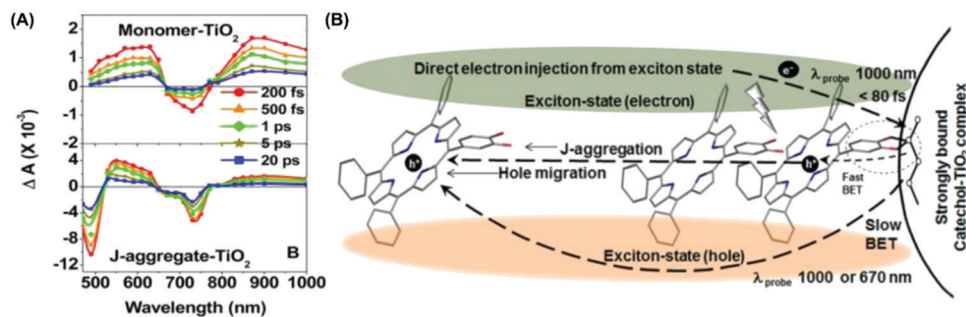
Fig. 27 (A) Distinction of absorption spectra between monomer- and J-aggregated porphyrin-TiO 2 NP 5 with different delay times. (B) Mechanism of charge-carrier shift in the J-aggregate porphyrin-TiO 2 system. Reprinted from ref. 403.
