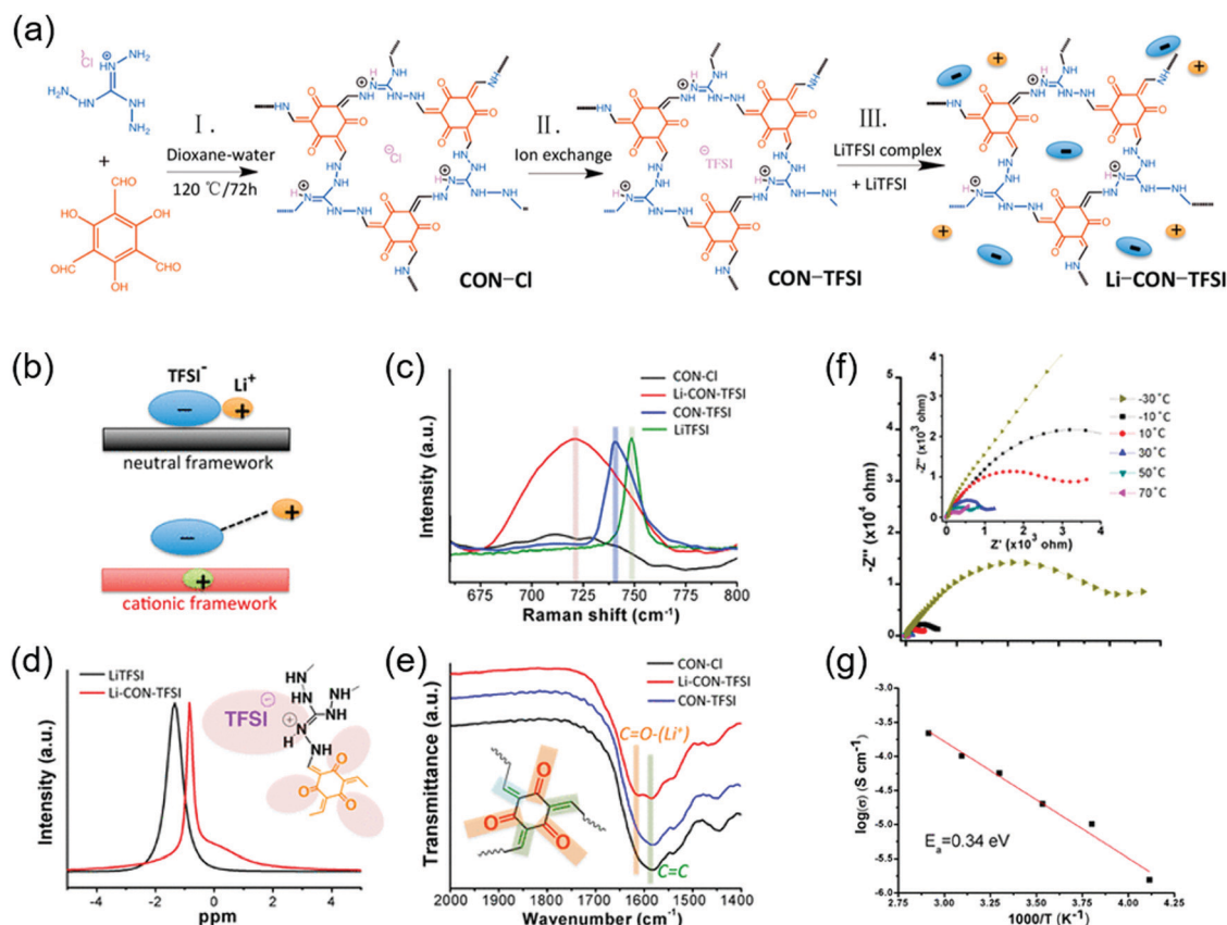
Fig. 21 Self-exfoliated, cationic COFs as \text{Li}^+ ion conductor. (a) Design and synthesis of cationic CONs for \text{Li}^+ conduction. (b) Differences in ion pair formation at neutral and cationic COF. (c) Raman spectra (d) ^7\text{Li} MAS NMR spectra (e) FTIR spectra of CONs and Li-CON-TFSI, establishing lithiation of CONs. (f) Temperature-dependent EIS of Li-CON-TFSI. (g) Calculation of activation energy ( E_a ) for Li-CON-TFSI in hydrous conditions by the methods of Arrhenius. Reproduced with permission. 154 Copyright 2018, American Chemical Society.
