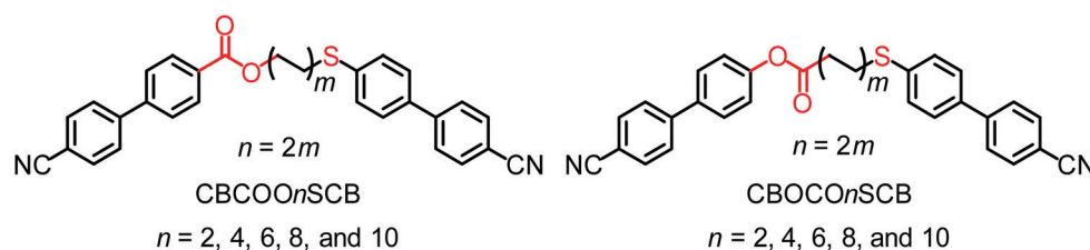
Fig. 1 Molecular structures of CBCOOnSCB ( n = 2, 4, 6, 8 , and 10 ) and CBOCOOnSCB ( n = 2, 4, 6, 8 , and 10 ), where n = 2m .
