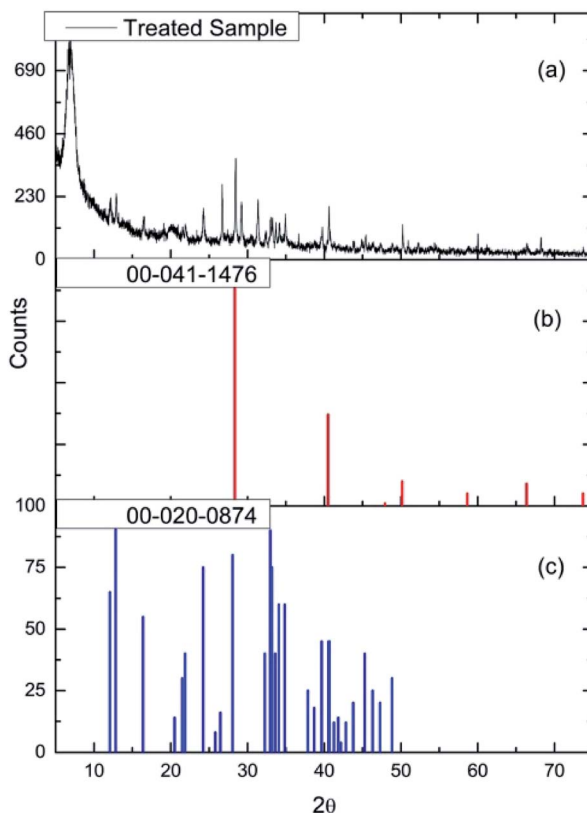
Fig. 15 (a) The X-ray diffraction pattern of the dichlorine pre-treated \text{CuCl}_2/\text{KCl}/\text{attapulgit} catalyst (chlorine exposure = 12.8 \text{ mmol Cl}_2 \text{ per g}_{(\text{cat})} ). Reference diffraction patterns for (b) KCl (red) and (c) \text{KCuCl}_3 (blue).
