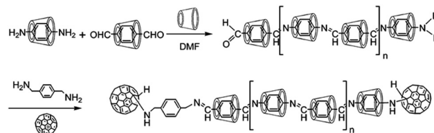
Scheme 18 Schematic representation of the synthesis of poly(azomethine) rotaxane capped with C_{60} as the end groups. The scheme has been reproduced from ref. 99 with permission from the American Chemical Society.
