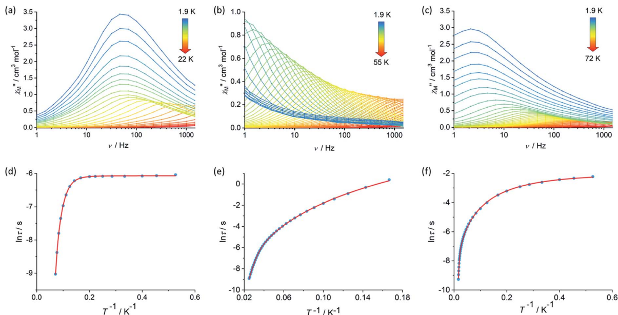
Fig. 2 Frequency dependence of the imaginary component of the AC susceptibility, \chi'' versus \nu , in zero DC field for (a) 1 , (b) 2 and (c) [3][B(C 6 F 5 ) 4 ] at the temperatures indicated, and the temperature dependence of the relaxation time as \ln \tau versus T^{-1} for 1 (d), 2 (e) and (f) [3][B(C 6 F 5 ) 4 ].
