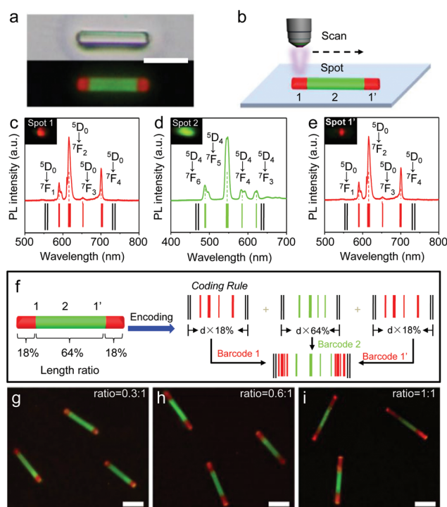
Fig. 8 (a) Bright-field and PL microscopy images of a segregated Ln-MOF heterostructure. Scale bar is 10\text{ }\mu\text{m} . (b) Schematic illustration of a heterostructure excited with a focused laser beam. Each part (marked as 1, 2, 1') of the heterostructure was selectively excited with a CW laser beam ( 375\text{ nm} ). (c–e) Corresponding PL spectra collected from three different areas and the generated barcodes (marked as 1, 2, 1' shown in b). (f) Schematic illustration of the encoding strategy based on the segregated Ln-MOF heterostructure. According to the different block lengths in a heterostructure, the as-designed barcodes were compressed with the corresponding length ratio, which can be defined as the sub-barcodes. The barcode was subsequently generated by combining the three parts of the sub-barcodes. (g–i) PL images of the segmented structure with various block lengths. The block length can be precisely controlled by adjusting the epitaxy precursor-to-seed ratio in the reaction system. Scale bars are 10\text{ }\mu\text{m} . Reproduced with permission from ref. 42. Copyright 2019, Wiley-VCH.
