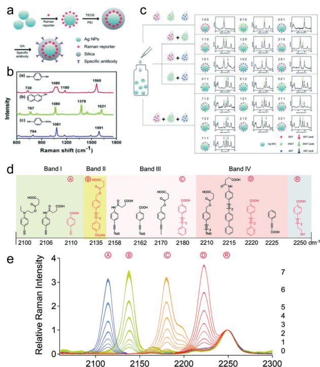
Fig. 7 (a) Schematic illustration of the preparation of the encoded SERS nanoprobes. Silver nanospheres were used as the SERS-active substrates, on which Raman reporters were adsorbed as the coding agents. Then, a layer of silica shell was coated for both protecting Raman reporters from the surroundings and providing a platform for further surface modifications. (b) SERS spectra of three SERS nanoprobes and the chemical structures of encoded Raman reporters: BDT, 2-NAT and 4-MT. (c) Codes, structures, and measured spectra of the synthesized 19 SERS encoders. The spectra are only shown from wavenumber 600 to 900 for clarity. (d) Molecular structures and Raman spectral properties of alkyne candidates for super-capacity coding systems. They are categorized into 4 spectral bands: bands I, II, III, and IV. Experimentally, these compounds labeled with \textcircled{A} , \textcircled{B} , \textcircled{C} , \textcircled{D} , and \textcircled{E} were selected to covalently attach to aminolated resin beads. (e) Eight Raman codes generated through mixing the compounds with different amount ratios. They correspond to \textcircled{A}_n ( n = 0-7 ) at 2110\text{ cm}^{-1} , \textcircled{B}_n ( n = 0-7 ) at 2135\text{ cm}^{-1} , \textcircled{C}_n ( n = 0-7 ) at 2180\text{ cm}^{-1} , and \textcircled{D}_n ( n = 0-7 ) at 2220\text{ cm}^{-1} , respectively. (a–c) Reproduced with permission from ref. 39. Copyright 2014, Royal Society of Chemistry. (d and e) Reproduced with permission from ref. 41. Copyright 2020, Royal Society of Chemistry.
