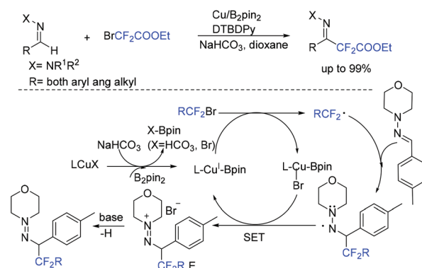
Scheme 113 The Cu/ \text{B}_2\text{pin}_2 -catalyzed difluoroalkylation of hydrazones.
