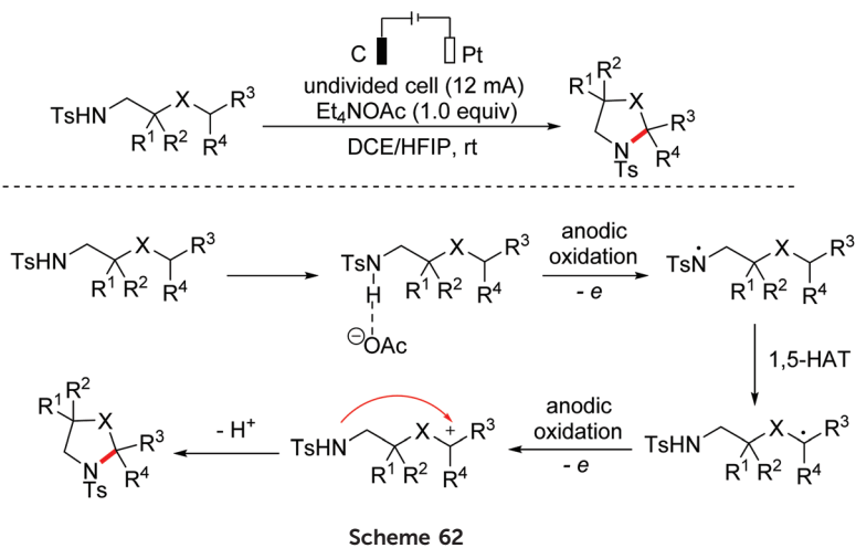
Scheme 62
