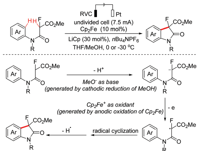
Scheme 56
