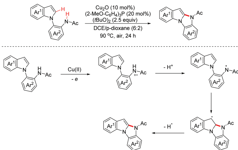
Scheme 61
