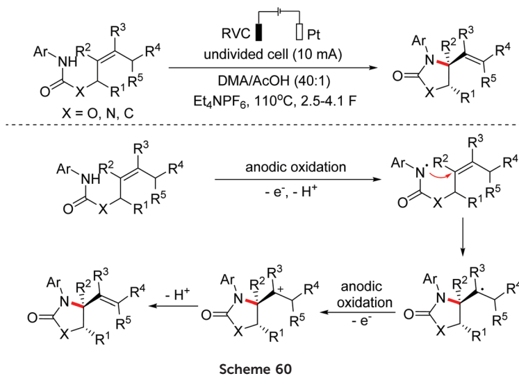
Scheme 60
