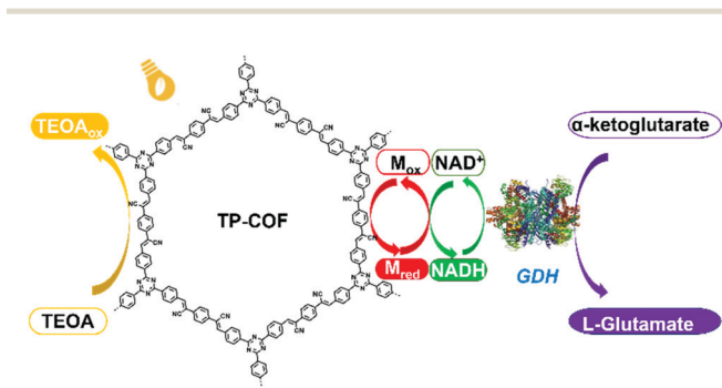
Fig. 10 Schematic illustration of the artificial photosystem I using TP-COF. Reproduced from ref. 117a with permission from Wiley-VCH Verlag GmbH & Co. KGaA, Copyright 2019.
