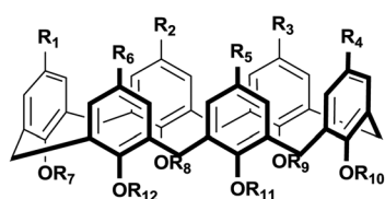
159: R_1=R_2=R_3=R_4=R_5=R_6=SO_3^- , R_7=R_8=R_9=R_{10}=R_{11}=R_{12}=C_3H_7
