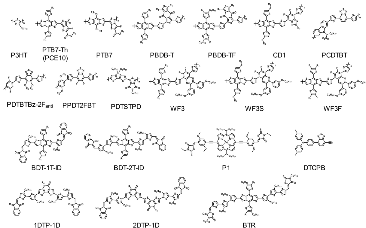
Fig. 3 Donor structures for indoor organic photovoltaic devices ( R_1 = 2-ethylhexyl, R_2 = 2-butyloctyl, R_3 = 2-hexyldecyl, R_4 = 2-octylidodecyl, R_5 = 2-decyltetradecyl).
