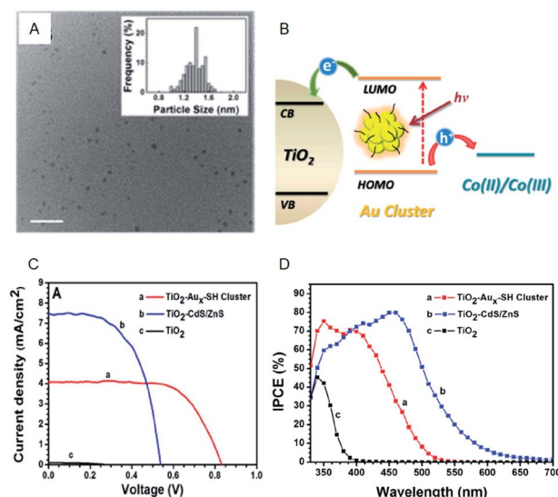
Fig. 13 (A) TEM image of \text{Au}_x -SG cluster. Scale bar shows the length of 10 nm. (B) Schematic of the working principle of metal-NC-sensitized solar cells. (C) J -V characteristics. (D) IPCE spectra of \text{TiO}_2 modified with \text{Au}_x -SH cluster, \text{TiO}_2 modified with CdS/ZnS and \text{TiO}_2 electrodes. Panels (a)–(d) are reproduced with permission from ref. 75. Copyright 2013 American Chemical Society.
