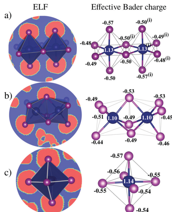
Fig. 4 Electron localization function (ELF) and effective Bader charge (e) of inorganic Bi_xI_y\delta^- moieties of perovskites (a) 1 , (b) 2 and (c) 3 . Along bismuth-iodide planes, the colors blue and red in the ELF plots represent electron charge depletion and accumulation, respectively.
