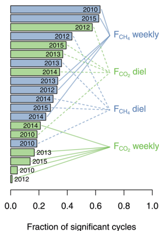
Fig. 5 Fraction of the time period covered in each year shown in Fig. 3 and 4 during which the diel or weekly cycle of the \text{CH}_4 and \text{CO}_2 fluxes were significant at p < 0.05 .
