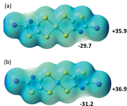
Fig. 9 Molecular electrostatic potential surfaces at the 0.001 \text{ e}^- \text{ au}^{-3} isodensity level for the neutral complexes \text{trans-}[\text{M}(\text{I-tzdt})_2] with (a) M = \text{Au} ; (b), M = \text{Ni} . Colour scale ranges from +36.89 \text{ kcal mol}^{-1} (blue) to -93.16 \text{ kcal mol}^{-1} (red).
