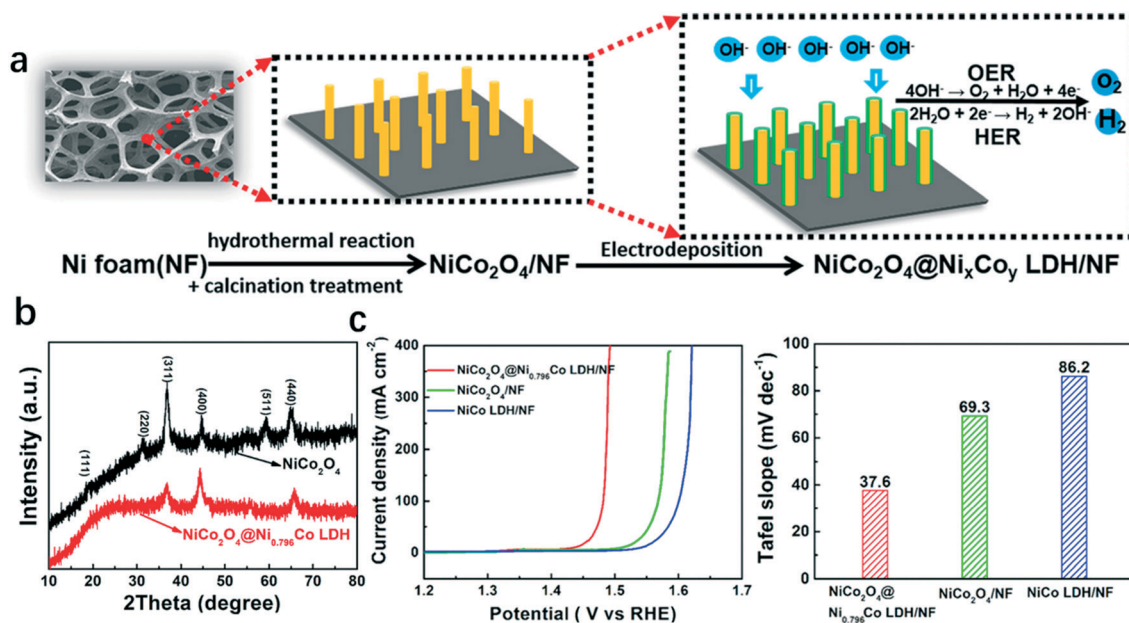
Fig. 2 Hybrid catalyst \text{NiCo}_2\text{O}_4@\text{Ni}_{0.796}\text{Co LDH/NF} with amorphous \text{Ni}_{0.796}\text{Co LDH} and crystallized \text{NiCo}_2\text{O}_4 as the shell and core, respectively. 37 (a) Illustration of the fabrication process of the hybrid catalyst, (b) XRD of \text{NiCo}_2\text{O}_4 and \text{NiCo}_2\text{O}_4@\text{Ni}_{0.796}\text{Co LDH} ; (c) polarization curves and Tafel slopes of \text{NiCo}_2\text{O}_4@\text{Ni}_{0.796}\text{Co LDH/NF} , \text{NiCo LDH/NF} , and \text{NiCo}_2\text{O}_4/\text{NF} .
