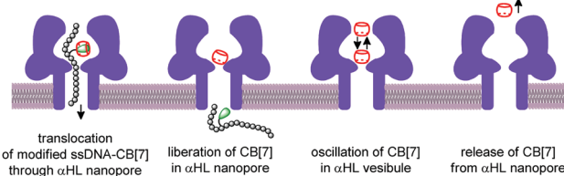
Fig. 3 Schematic representation of the CB-assisted nanopore sensing, including the trapping of the DNA probe, its dissociation, translocation, and CB[7] oscillation in the vestibule of the \alpha -hemolysin nanopore.
