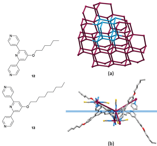
Fig. 10 Structures of ditopic ligands 12 and 13 . (a) Part of the neb net in [\text{Co}(\text{NCS})_2(\mathbf{12})]_n showing the Co nodes. One 6^6 unit of the neb topology is highlighted in blue. (CSD refcode EMEJIR, TOPOS 49 representation.) (b) The octahedral coordination geometry of the trans - \{\text{Co}(\text{NCS})_2\text{N}_4\} unit places the pyridine N-donors in a plane (in blue), but the Co node in the network is topographically tetrahedral (maroon connections).
