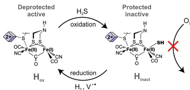
Scheme 1 Protection of DdHdAB with sulfide under oxidative conditions and its reactivation in a redox film under reductive conditions.
