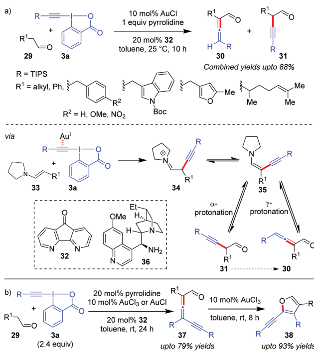
Scheme 7 (a) \alpha -Vinylidene of aliphatic aldehydes using a Au/pyrrolidine catalyst system; and (b) one-pot relay of \alpha -vinylidene/ \gamma -alkynylation of aliphatic aldehydes.
