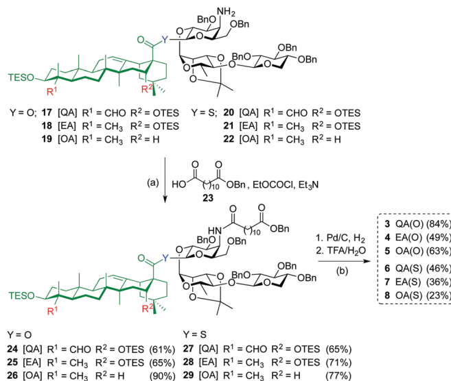
Scheme 2 Reagent and conditions: (a) EtOCCl, \text{Et}_3\text{N} , THF, 0 °C to r.t., 4 h, 61% (for 24 ), 65% (for 25 ), 90% (for 26 ); 65% (for 27 ), 71% (for 28 ), and 77% (for 29 ); (b) 1: Pd/C, \text{H}_2 (1 atm), EtOH/THF 1 : 1, r.t., 16 h (for 24–26 ); 20 min (for 27–29 ); 2: TFA/ \text{H}_2\text{O} 3 : 1, 0 °C, 1 h, 84% (for 3 ), 49% (for 4 ), 63% (for 5 ); 46% (for 6 ), 36% (for 7 ), and 23% (for 8 ).
