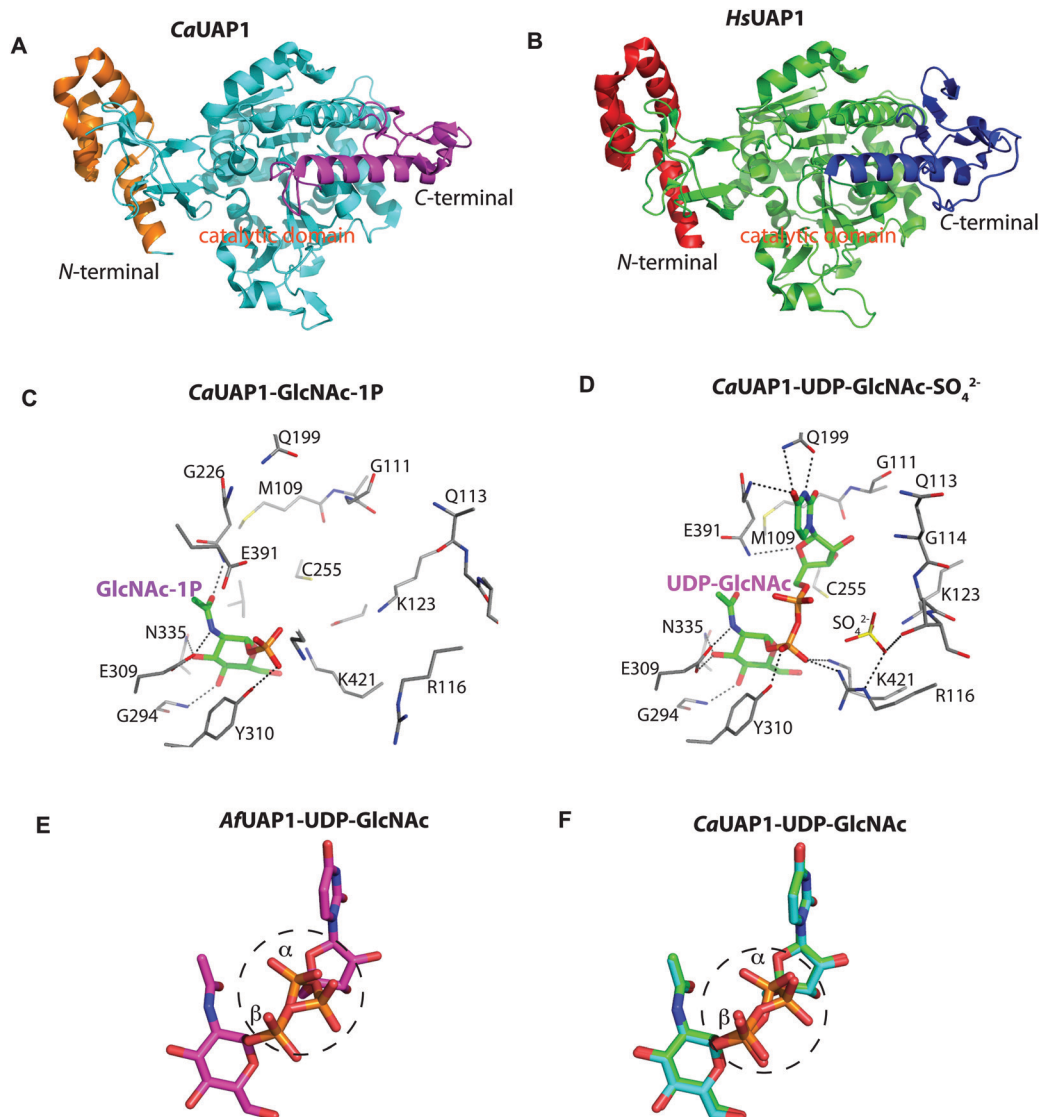
Fig. 3 Comparison of AfUAP1 with other UAP1s. (A) Overall structure of CaUAP1. Coloured in orange, cyan and purple are the N-terminal, catalytic and C-terminal domains, respectively. (B) Overall structure of HsUAP1. Coloured in red, green and blue are the N-terminal, catalytic and C-terminal domains, respectively. (C) Active site of CaUAP1 with GlcNAc-1P bound. Active site residues are shown in sticks. Hydrogen bond interactions are shown as black dashes. (D) Active site of CaUAP1 with UDP-GlcNAc-SO 4 2- bound. Active site residues are shown in sticks. Hydrogen bond interactions are shown as black dashes. SO 4 2- is shown as sticks. (E) Stick representation of UDP-GlcNAc in the AfUAP1-UDP-GlcNAc-Pi-Mg 2+ ternary complex, showing the observed dual conformation around the \alpha -phosphate. (F) Superposition of UDP-GlcNAc from the CaUAP1-UDP-GlcNAc product complex (PDB: 2yqs, blue) with UDP-GlcNAc from the CaUAP1-UDP-GlcNAc reaction-completed product complex (PDB: 2yqj, green). This superposition recapitulates the dual conformation observed in the AfUAP1-UDP-GlcNAc-Pi-Mg 2+ complex.
