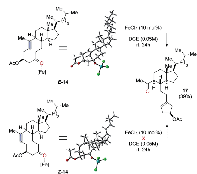
Fig. 6 Comparison of reactivity between E and Z isomers of cholesterol-derived substrate 14 .
