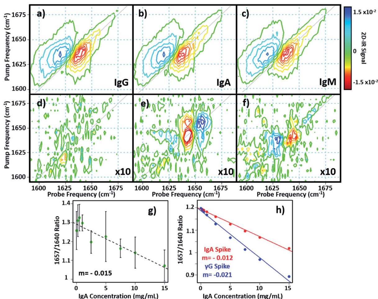
Fig. 6 (a–c) 2D-IR spectra of IgG, IgA and IgM in H 2 O. (d–f) Difference spectra obtained by subtracting the 2D-IR response of the spectra in (a–c) from that of the γ-globulins. The spectral features have been magnified by a factor of 10 for clarity and are shown on the same scale as (a–c). (g and h) show the variation in 2D-IR signal at the peak of the difference spectral response for IgA as a function of added protein for the experimental data (g) and calculations (h). The linear increase in the negative signal shows a correlation with protein content.
