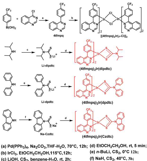
Scheme 1 The synthetic routes to the ligands and complexes.
