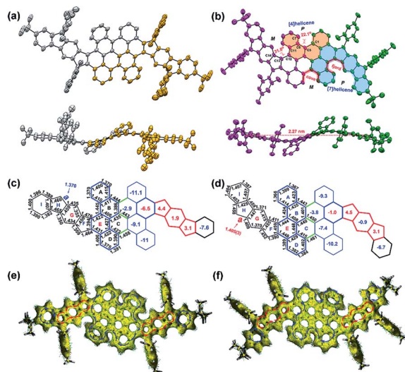
Fig. 3 Top view and side view of the X-ray crystallographic structure of (a) compound 1 (precursor for PH 1) and (b) tetraradicaloid 2; the hydrogen atoms are omitted for clarity. Selected bond lengths (Å) and calculated NICS(1) av values in the rings A–I of (c) 1 and (d) 2. Calculated ACID plots of (e) 1 and (f) 2. Isovalue is 0.05, and the blue and red arrows indicate diamagnetic and paramagnetic ring current flows, respectively.
