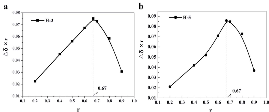
Fig. 3 ^1\text{H} NMR Job's curves base on H-3 (a), and H-5 (b) of \beta -CD in \text{D}_2\text{O} .
