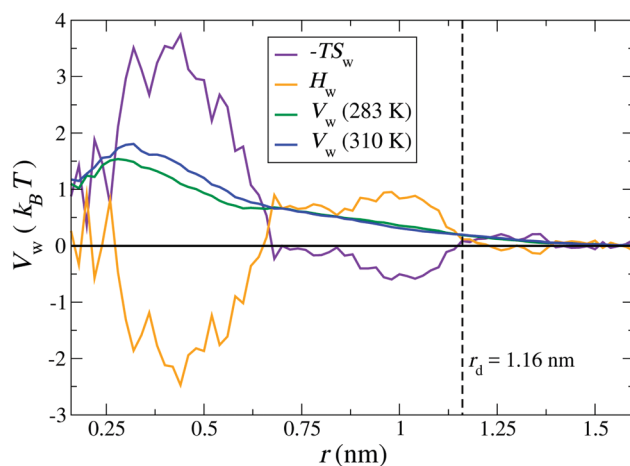
Fig. 6 Distance-resolved thermodynamic profiles for water binding to the G2-dPGS. The potential of mean force V_w(r) is shown at 283 K and 310 K. The entropic profile -TS_w and the enthalpy profile H_w were calculated from the two PMFs by a finite difference derivative [eqn (11)] and the standard thermodynamic relation, eqn (12), at the mean temperature 296.5 K. The dashed vertical line indicates the bare radius r_d of G2-dPGS.
