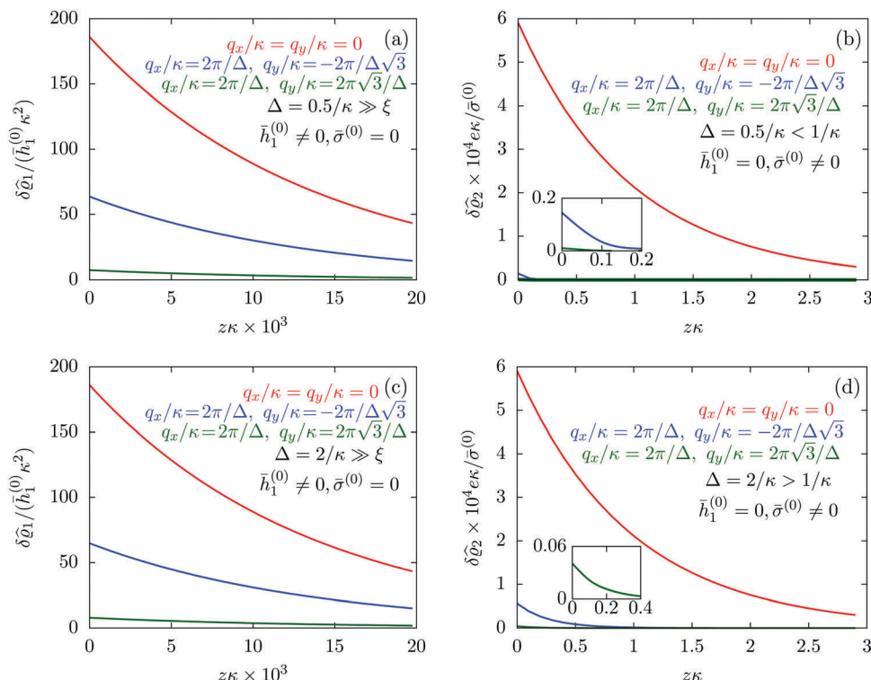
Fig. 7 Density profiles of the solvent (panels (a) and (c)) and of the ions (panels (b) and (d)) for three lateral wave vectors \mathbf{q}_{||} = (q_x, q_y) as functions of the normal distance z from the wall in units of the Debye length 1/\kappa . The boundary condition corresponds to a hexagonal lattice of interaction sites with a Gaussian charge distribution characterized by a standard deviation \Delta_{\text{peaks}} = \Delta/5 . The lattice constant is denoted as \Delta (see Fig. 5). In panels (a) and (b) the lattice constant and the variance are \Delta = 0.5/\kappa and \Delta_{\text{peaks}} = 0.1/\kappa , respectively, whereas in panels (c) and (d) the lattice constant and the variance are \Delta = 2/\kappa and \Delta_{\text{peaks}} = 0.4/\kappa , respectively, with the Debye length 1/\kappa (see eqn (34)). Panels (a) and (c) correspond to systems with a nonelectrostatic interaction between the wall and the solvent particles (see eqn (56)), whereas panels (b) and (d) correspond to systems with electrostatic interaction sites between wall and ions (see eqn (57)). The insets in (b) and (d) show a magnified version of the respective profiles in the main plot. In all cases, the profiles decay exponentially upon increasing the normal distance z from the wall. However, the decay length differs significantly between the two aforementioned types of interactions. In the case of the nonelectrostatic interaction, the decay length is set by the bulk correlation length \xi (see eqn (36)) of the fluid, whereas in the case of the electrostatic interaction it is set by the much larger Debye length 1/\kappa . This difference in the decay lengths, both in lateral and in normal direction, which leads to a much faster lateral decay in the case of the electrostatic interactions, is also responsible for the decreasing amplitude of the ion profiles for increased wave vectors (panel (b) and (d)). Another significant difference between the two interaction types is the variation of the decay length as function of the lateral wave vectors. In panels (a) and (c) all profiles decay exponentially on the same decay length \xi , whereas in panels (b) and (d) the decay length depends significantly on the wave vectors. This effect follows from the dependence of the eigenvalues on |\mathbf{q}_{||}| as discussed in eqn (A3), corresponding to a lateral decay proportional to \exp(-\sqrt{\kappa^2 + |\mathbf{q}_{||}|^2}z) . In principle this occurs for both types of interactions. However only in the case of the electrostatic interactions it is relevant, which again is due to the difference between the dominating length scales. For the remaining relevant parameters see Section IIIA.
