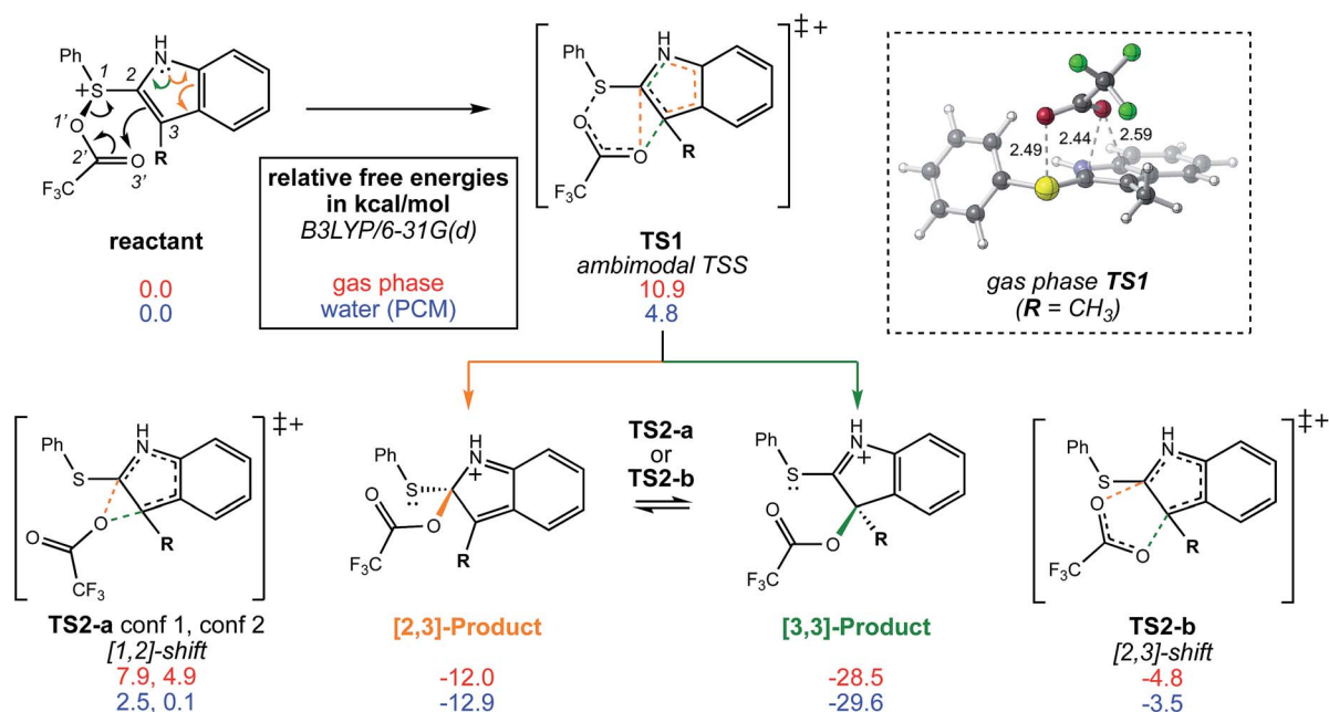
Fig. 2 The bifurcating reaction scheme investigated in this study, along with a CYLview 14 image of TS1 in the gas phase showing the tri-fluoroacetyl oxygen's approach to the \pi -bond of the indole ring. The atom numbers shown do not correspond to those used to name the sigmatropic shifts. Relative free energies shown are for stationary points optimized in the gas phase (red) and in water using a polarized continuum solvent model (PCM, blue). Stationary points were optimized at the B3LYP/6-31G(d) level of theory.
