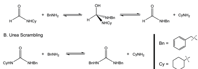
Scheme 2 Potential scrambling pathways in unsymmetric urea formation.
