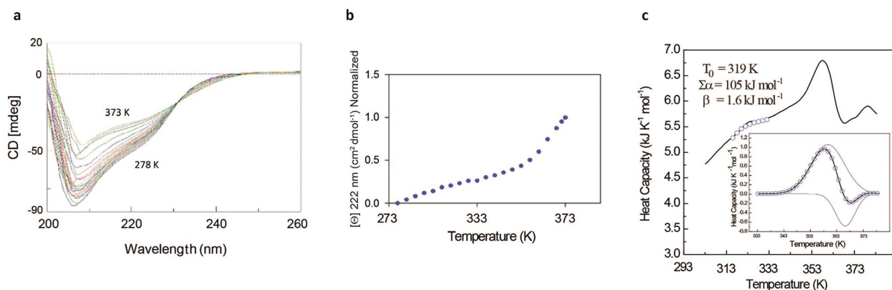
Fig. 4 Ml1 53–149 unfolding behavior. (a) Thermal unfolding of Ml1 53–149 in the range 278–373 K at regular intervals of 3 K: the figure shows the isodichroic point at 233 nm observable in the range of 278–353 K. (b) Melting curve monitored by CD at 222 nm. (c) Representative profile of thermally induced unfolding of Ml1 53–149 monitored by DSC.
