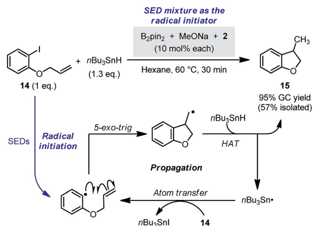
Scheme 12 Radical chain reaction initiated by the diboron-derived SEDs.
