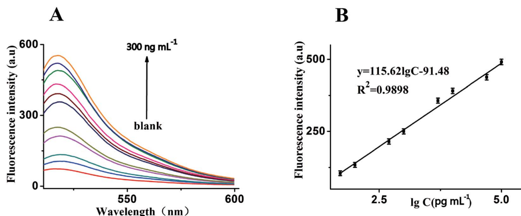
Fig. 5 (A) Fluorescence emission spectra of the biosensor in the presence of MUC1 with different concentrations: from bottom to top: 0, 10 \text{pg mL}^{-1} , 50 \text{pg mL}^{-1} , 100 \text{pg mL}^{-1} , 500 \text{pg mL}^{-1} , 1 \text{ng mL}^{-1} , 5 \text{ng mL}^{-1} , 10 \text{ng mL}^{-1} , 50 \text{ng mL}^{-1} , 100 \text{ng mL}^{-1} , 200 \text{ng mL}^{-1} and 300 \text{ ng mL}^{-1} , respectively. (B) The relationship curve of the fluorescence intensity as a function of MUC1 concentration. While shows the relationship between fluorescence intensity and MUC1 concentration, both experimental conditions: Dnase I, 2 \text{ U mL}^{-1} ; MUC1, 5 \text{ ng mL}^{-1} ; probe, 40 \text{ nM} ; GO, 15 \mu\text{g mL}^{-1} and the emission wavelength of 519 \text{ nm} . Error bars: SD, n = 3 .
