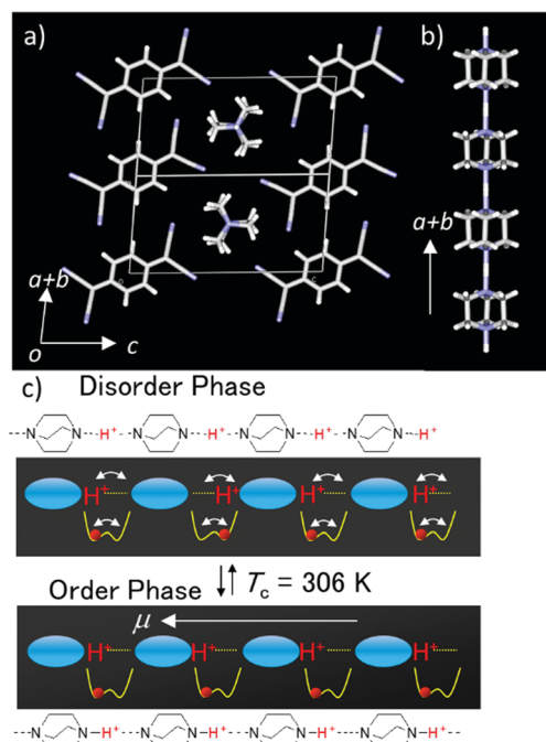
Fig. 3 Dynamic short-range collective proton transfer and dielectric switching in the organic semiconductor (HDABCO ^+ ) 2 (TCNQ) 3 . (a) Unit cell viewed along the 1D (N–H ^+ ...N) _{\infty} hydrogen-bonding chain and electrical conducting \pi -column of TCNQ. (b) High temperature 1D (N–H ^+ ...N) _{\infty} hydrogen-bonding chain of HDABCO ^+ cations along the a + b axis. Schematic potential energy curves of the N–H ^+ ...N hydrogen-bonding chain (c) at the high temperature paraelectric disordered phase (upper) and at the low temperature ordered ferroelectric phase (lower) for the proton orientation.
