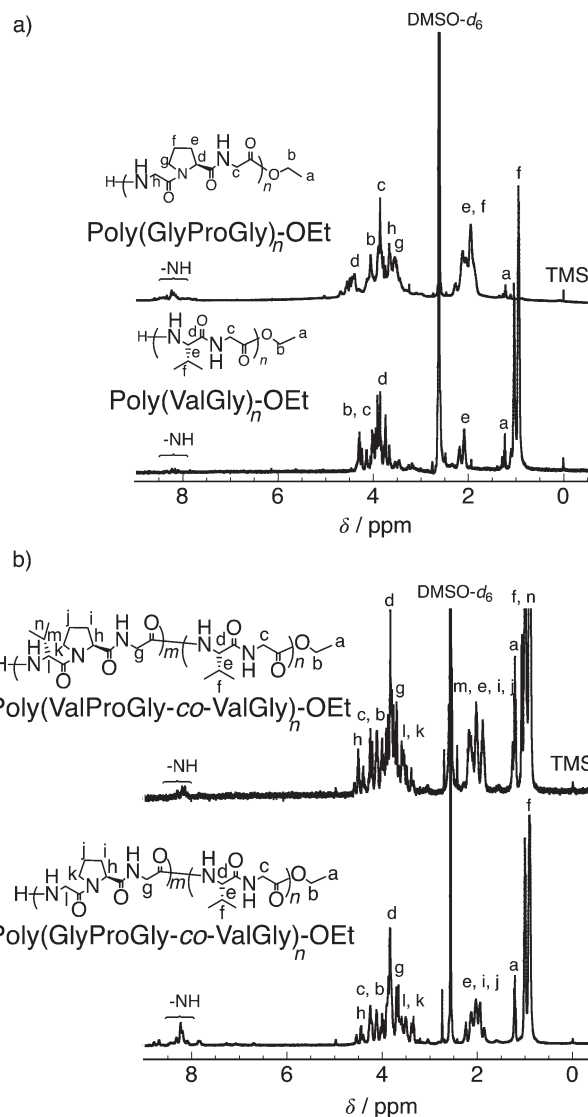
Fig. 2 ^1\text{H} NMR spectra of (a) poly(GlyProGly) and poly(ValGly) and (b) poly(ValProGly-co-ValGly) and poly(GlyProGly-co-ValGly), in \text{DMSO}-d_6/\text{TFA}-d (5/1).
