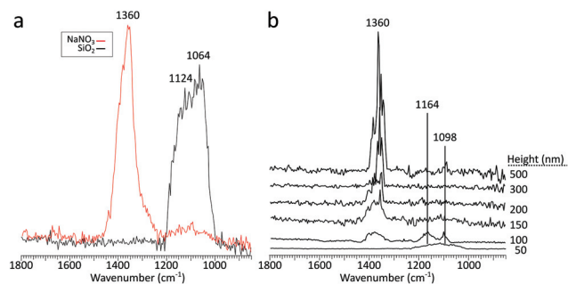
Fig. 9 (a) PTIR spectra obtained on a NaNO 3 particle (red) and silicon substrate (black), (b) PTIR spectra taken for particles of varying height.
