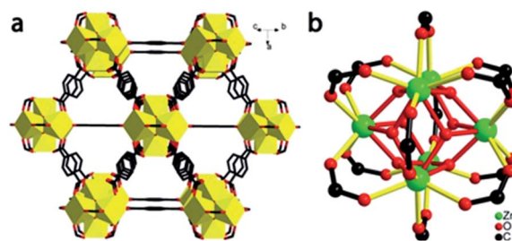
Fig. 1 Structure of UiO-66. (a) Extended 3D structure, showing the bridging terephthalates ligated to zirconia clusters. (b) Coordination geometry around the \text{Zr}_6\text{O}_4(\text{OH})_4(\text{O}_2\text{CR})_{12} clusters.
