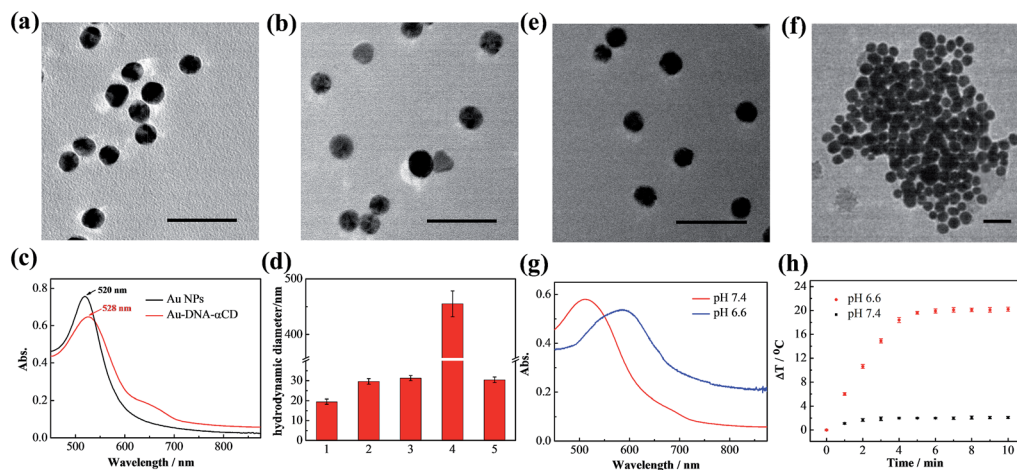
Fig. 1 Characterization of the gold nanomachines and in vitro verification of the fabrication of the gold nanomachines triggered by the mildly acidic environment. High-resolution transmission electron microscopy images of (a) AuNPs and (b) Au-DNA- \alpha CDs. Scale bar represents 50 nm. (c) Absorption spectra of AuNPs and Au-DNA- \alpha CDs. An 8 nm red-shift is apparent after DNA modification and \alpha -CD capping. (d) Hydrodynamic diameters of different samples measured by DLS: (1) AuNPs; (2) Au-DNA- \alpha CD; (3) and (4) Au-DNA- \alpha CDs at pH 7.4 or 6.6, respectively, in PBS buffer (10 mM, Na + (10 mM) and Mg 2+ (5 mM)); (5) Au-DNA- \alpha CDs in PBS buffer (10 mM, Na + (10 mM), Mg 2+ (5 mM), Ca 2+ (0.5 mM) and DNase I (2 U L -1 )) at pH 7.4. (e and f) High-resolution transmission electron microscopy images of the gold nanomachines incubated at pH 7.4 and 6.6 in PBS buffer. Scale bar represents 50 nm. (g) Absorption spectra of gold nanomachines at pH 7.4 and 6.6. The absorption spectrum of the gold aggregates shows a substantial red-shift and possesses a wide range of NIR absorption. (h) Temperature elevation of the gold nanomachines at pH 6.6 or 7.4 as a function of irradiation time. The temperature of the gold nanomachines at pH 6.6 reached 45 °C after irradiation, whereas less than a 3 °C increase was observed at pH 7.4.
