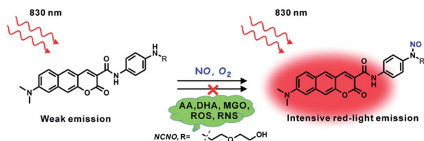
Scheme 1 Schematic of the N -nitrosation-reactivity-based two-photon fluorescent probe NCNO for NO.
