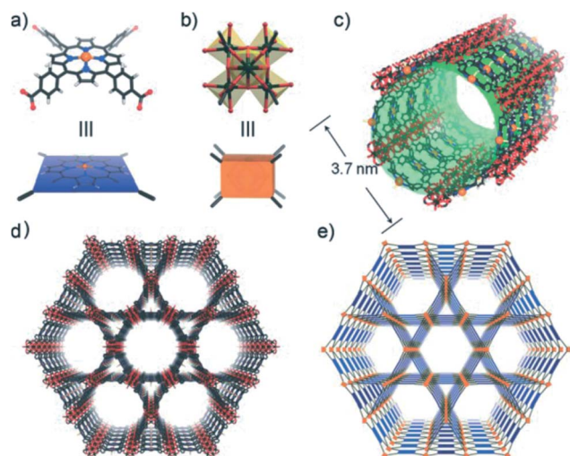
Fig. 1 The crystal structure and underlying network topology of PCN-222(Fe). The \text{Fe}-\text{L}^1 (a; blue square) is connected to four 8-connected \text{Zr}_6 clusters (b; light orange cuboid), generating a 3D network with Kagome-like topology (d, e) and large 1D channels (c; green pillar). Zr: black spheres, C: gray, O: red, N: blue, and Fe: orange. [Reprinted with permission from ref. 56. Copyright 2012, Wiley-VCH Verlag GmbH & Co. KGaA, Weinheim.]
