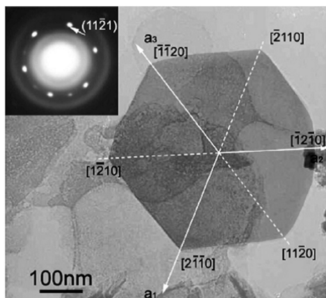
Fig. 4 TEM image and selected area electron diffraction (SAED) pattern (inset) of a regular hexagonal Mg(OH) 2 nanoflake synthesised from Mg(NO 3 ) 2 and N 2 H 4 ·H 2 O. Reprinted from Materials Chemistry and Physics , 112 , D. Jin, X. Gu, X. Yu, G. Ding, H. Zhu and K. Yao, Hydrothermal synthesis and characterization of hexagonal Mg(OH) 2 nano-flake as a flame retardant, 962–965, copyright 2008, with permission of Elsevier. 31
