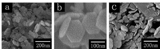
Fig. 5 SEM images of Mg(OH) 2 nanoflakes (a) synthesised with PEG20000 (at low magnification); (b) synthesised with PEG20000 (at higher magnification) and (c) synthesised without PEG 20000. Reprinted from Materials Research Bulletin , 51 , Q. Wang, C. Li, M. Guo, L. Sun and C. Hu, Hydrothermal synthesis of hexagonal magnesium hydroxide nanoflakes, 35–39, copyright 2014, with permission of Elsevier. 32
