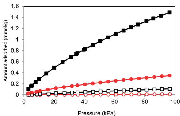
Fig. 3 \text{CO}_2 and \text{N}_2 adsorption isotherms for 1 and 2 at 0 °C (black squares, \text{CO}_2 for 1 ; open squares, \text{N}_2 for 1 ; red circles, \text{CO}_2 for 2 ; open circles, \text{N}_2 for 2 ).
