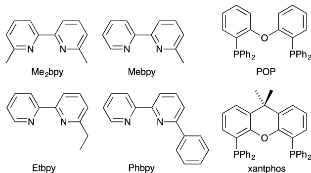
Scheme 1 Structures of \text{N}^*\text{N} ligands 6,6'-dimethyl-2,2'-bipyridine ( \text{Me}_2\text{bpy} ), 6-methyl-2,2'-bipyridine (Mebpy), 6-ethyl-2,2'-bipyridine (Etbpy) and 6-phenyl-2,2'-bipyridine (Phbpy), and the \text{P}^*\text{P} ligands POP and xantphos.
