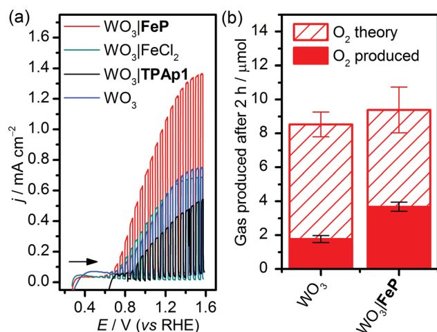
Fig. 3 (a) LSVs under chopped illumination ( \text{AM1.5G} , 0.2\text{ W cm}^{-2} ) of \text{WO}_3 (blue line), \text{WO}_3|\text{FeP} (red line), \text{WO}_3|\text{FeCl}_2 (green line) and \text{WO}_3|\text{TPAp1} (black line) at \nu = 5\text{ mV s}^{-1} . (b) Amount of \text{O}_2 generated after two h PEC water oxidation by nano \text{WO}_3 with and without FeP under solar illumination at E_{\text{appl}} = 1.0\text{ V} vs. RHE. The theoretical amount of \text{O}_2 was calculated based on 100% faradaic yield and the experimentally measured \text{O}_2 was quantified by a fluorescence probe. Conditions: a Ag/AgCl reference electrode and a Pt mesh counter electrode in aqueous \text{Na}_2\text{SO}_4 (0.1 M) solution at pH 3, \text{N}_2 atmosphere and room temperature.
