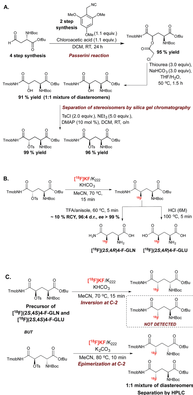
Scheme 2 (A.) Synthesis of the substrates for the radiosynthesis of ^{18}\text{F} -GLU and ^{18}\text{F} -GLN. (B.) Radiosynthesis of ^{18}\text{F} -(2S,4R)-4F-GLU and ^{18}\text{F} -(2S,4R)-4F-GLN. (C.) Radiosynthesis of ^{18}\text{F} -(2S,4S)-4F-GLU and ^{18}\text{F} -(2S,4S)-4F-GLN precursors. Tmob = 2,4,6-trimethoxybenzyl.
