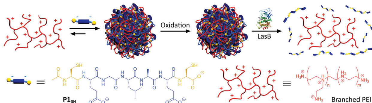
Scheme 1 Assembly and oxidative cross-linking of PIC nanoparticles from \text{P1}_{\text{SH}} (Ac-C-E-GLA-E-C-OH) and antimicrobial branched PEI. Degradation of PIC nanoparticles by LasB and subsequent PEI release.
